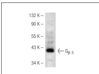
G β5 (N-20): sc-25025. Western blot analysis of G β5 expression in mouse brain tissue extract.
