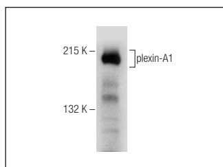
plexin-A1 (S-16): sc-10139. Western blot analysis of plexin-A1 expression in K-562 whole cell lysate.
