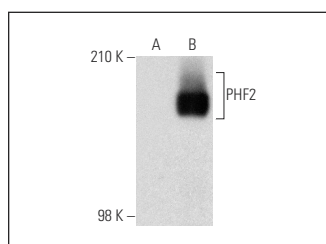
PHF2 (I-13): sc-101864. Western blot analysis of PHF2 expression in non-transfected: sc-117752 (A) and mouse PHF2 transfected: sc-122538 (B) 293T whole cell lysates.
