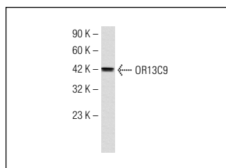
OR13C9 (S-22): sc-102047. Western blot analysis of OR13C9 expression in Hep G2 whole cell lysate.
