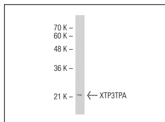
XTP3TPA (G-23): sc-102159. Western blot analysis of XTP3TPA expression in Hep G2 whole cell lysate.
