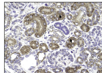
XTP3TPA (G-23): sc-102159. Immunoperoxidase staining of formalin fixed, paraffin-embedded human kidney tissue showing cytoplasmic staining.
