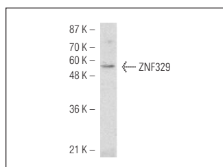
ZNF329 (M-18): sc-102208. Western blot analysis of ZNF329 expression in Hep G2 whole cell lysate.
