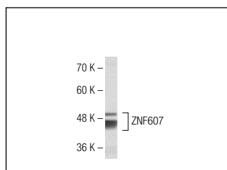
ZNF607 (K-25): sc-102250. Western blot analysis of ZNF607 expression in Jurkat whole cell lysate.
