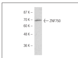
ZNF750 (M-23): sc-102269. Western blot analysis of ZNF750 expression in Hep G2 whole cell lysate.
