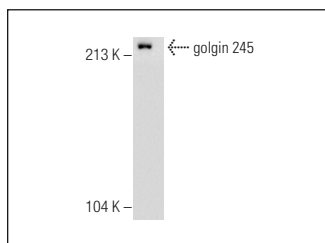
golgin 245 (N-16): sc-102566. Western blot analysis of golgin 245 expression in T-47D whole cell lysate.
