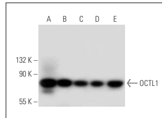
OCTL1 (N-15): sc-103090. Western blot analysis of OCTL1 expression in C6 (A), KNRK (B), HL-60 (C), Hep G2 (D) and HeLa (E) whole cell lysates.
