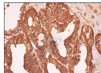
SNX5 (D-18): sc-10625. Immunoperoxidase staining of formalin fixed, paraffin-embedded human seminal vesicle tissue showing cytoplasmic and membrane staining of glandular cells.
