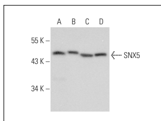
SNX5 (D-18): sc-10625. Western blot analysis of SNX5 expression in A549 (A), U-251-MG (B), Jurkat (C) and HEK293 (D) whole cell lysates.
