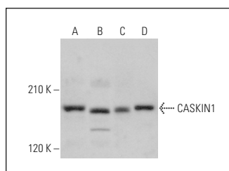
CASKIN1 (S-17): sc-107181. Western blot analysis of CASKIN1 expression in K-562 (A), HeLa (B), MOLT-4 (C) and PC-3 (D) whole cell lysates.
