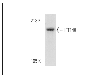
IFT140 (K-14): sc-107624. Western blot analysis of IFT140 expression in ARPE-19 whole cell lysate.
