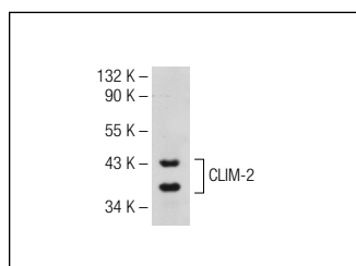
CLIM-2 (T-16): sc-11199. Western blot analysis of CLIM-2 expression in HeLa nuclear extract.
