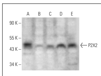
P2X2 (V-17): sc-12211. Western blot analysis of P2X2 expression in Hep G2 (A), Jurkat (B), HeLa (C), MCF7 (D) and K-562 (E) whole cell lysates.
