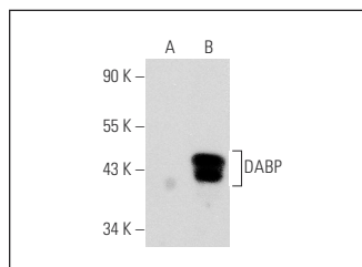
DABP (E-13): sc-131141. Western blot analysis of DABP expression in non-transfected: sc-117750 (A) and human DABP transfected: sc-112971 (B) whole cell lysates.
