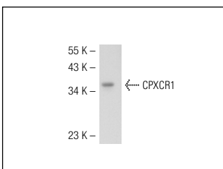
CPXCR1 (F-13): sc-131467. Western blot analysis of CPXCR1 expression in mouse embryo tissue extract.
