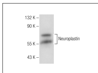
Neuroplastin (S-12): sc-131990. Western blot analysis of Neuroplastin expression in mouse brain tissue extract.
