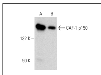
CAF-1 p150 (C-5): sc-133068. Western blot analysis of CAF-1 p150 expression in Jurkat nuclear extract (A) and HeLa whole cell lysate (B).
