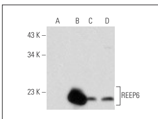
REEP6 (C-13): sc-133408. Western blot analysis of REEP6 expression in non-transfected 293T: sc-117752 (A), human REEP6 transfected 293T: sc-110960 (B), Hep G2 (C) and PC-3 (D) whole cell lysates.
