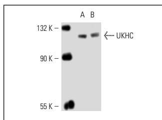
UKHC (C-15): sc-13359. Western blot analysis of UKHC expression in HeLa (A) and KNRK (B) whole cell lysates.
