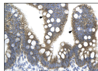
TFB2M (X-23): sc-134078. Immunoperoxidase staining of formalin-fixed, paraffin-embedded human intestine tissue showing cytoplasmic localization.
