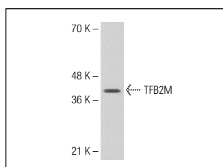
TFB2M (X-23): sc-134078. Western blot analysis of human TFB2M transfected 293T whole cell lysate.
