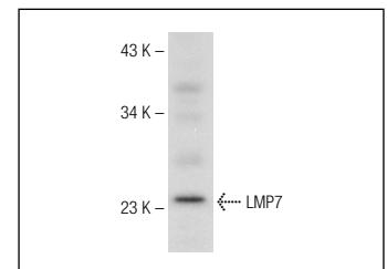
LMP7 (H-40): sc-134503. Western blot analysis of LMP7 expression in MOLT-4 whole cell lysate.
