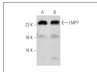
LMP7 (H-40): sc-134503. Western blot analysis of LMP7 expression in CCRF-CEM (A) and HuT 78 (B) whole cell lysates.
