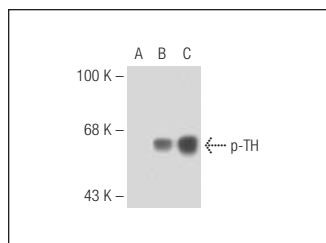
p-TH (Ser 19): sc-135713. Western blot analysis of TH phosphorylation in purified non-phosphorylated rat recombinant TH fusion protein (A) and untreated PC-12 (B) and KCl-stimulated PC-12 (C) whole cell lysates.
