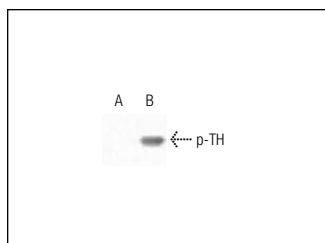
p-TH (Ser 40): sc-135715. Western blot analysis of non-phosphorylated (A) and phosphorylated (B) rat recombinant TH fusion proteins.
