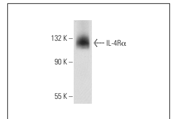
IL-4R \alpha (G-9): sc-137256. Western blot analysis of IL-4R \alpha expression in NIH/3T3 whole cell lysate.
