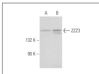
ZZZ3 (D-13): sc-137963. Western blot analysis of ZZZ3 expression in HEK293 (A) and Jurkat (B) whole cell lysates.
