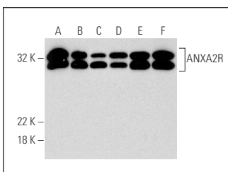
ANXA2R (D-12): sc-137985. Western blot analysis of ANXA2R expression in K-562 (A), HEK293 (B), HeLa (C), SUP-T1 (D), Jurkat (E) and HuT 78 (F) whole cell lysates.
