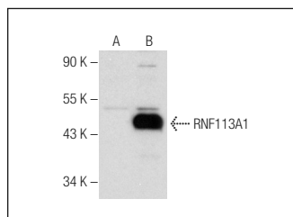
RNF113A (C-13): sc-138587. Western blot analysis of RNF113A1 expression in non-transfected: sc-117752 (A) and mouse RNF113A1 transfected: sc-123229 (B) 293T whole cell lysates.
