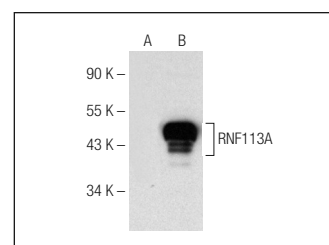
RNF113A (E-15): sc-138588. Western blot analysis of RNF113A expression in non-transfected: sc-117752 (A) and mouse RNF113A transfected: sc-123229 (B) 293T whole cell lysates.
