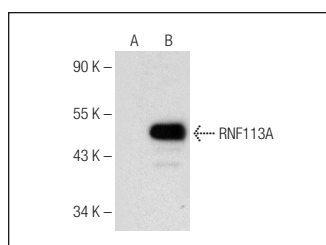
RNF113A (E-15): sc-138588. Western blot analysis of RNF113A expression in non-transfected: sc-117752 (A) and human RNF113A transfected: sc-112744 (B) 293T whole cell lysates.
