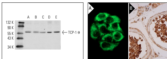
TCP-1 \theta (N-18): sc-13891. Western blot analysis of TCP-1 \theta expression in F9 (A), HeLa (B) and Jurkat (C) whole cell lysates and rat (D) and mouse (E) testis extracts
