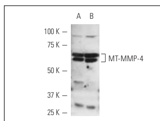
MT-MMP-4 (H-110): sc-13972. Western blot analysis of MT-MMP-4 expression in MCF7 (A) and LNCaP (B) whole cell lysates.
