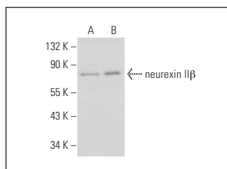
neurexin II \beta (H-15): sc-14345. Western blot analysis of neurexin II \beta expression in C6 (A) and PC-12 (B) whole cell lysates.
