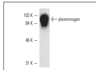
plasminogen (H-14): sc-15033. Western blot analysis of human recombinant plasminogen.
