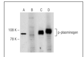
Western blot analysis of plasminogen phosphorylation in untreated (A,C) and lambda protein phosphatase (sc-200312A) treated (B,D) human platelet extracts. Antibodies tested include p-plasminogen (Ser 578)-R: sc-16310-R (A,B) and plasminogen (H-14): sc-15033 (C,D).
