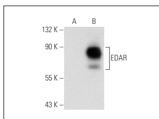
EDAR (C-20): sc-15290. Western blot analysis of EDAR expression in non-transfected: sc-117752 (A) and human EDAR transfected: sc-177166 (B) 293T whole cell lysates.
