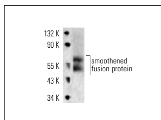
smoothened (dC-20): sc-15671. Western blot analysis of Drosophila recombinant smoothened fusion protein.
