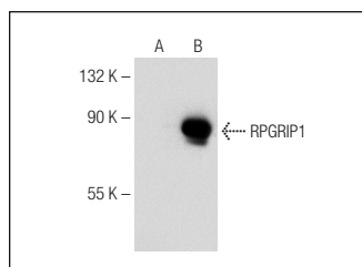
RPGRIP1 (E-14): sc-160753. Western blot analysis of RPGRIP1 expression in non-transfected: sc-117752 (A) and mouse RPGRIP1 transfected: sc-123274 (B) 293T whole cell lysates.
