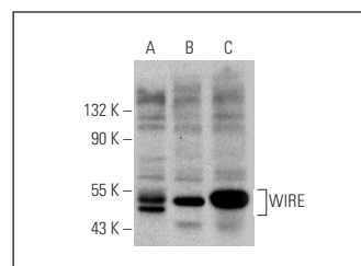
WIRE (P-13): sc-160920. Western blot analysis of WIRE expression in ES-2 (A), MCF7 (B) and SK-BR-3 (C) whole cell lysates.
