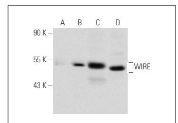
WIRE (P-13): sc-160920. Western blot analysis of WIRE expression in non-transfected 293T: sc-117752 (A), human WIRE transfected 293T: sc-117025 (B), SK-BR-3 (C) and Ramos (D) whole cell lysates.
