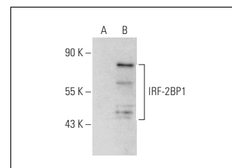
IRF-2BP1 (T-14): sc-161745. Western blot analysis of IRF-2BP1 expression in non-transfected: sc-117752 (A) and human IRF-2BP1 transfected: sc-114866 (B) 293T whole cell lysates.
