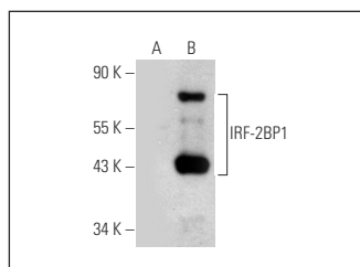
IRF-2BP1 (T-14): sc-161745. Western blot analysis of IRF-2BP1 expression in non-transfected: sc-117752 (A) and human IRF-2BP1 transfected: sc-111584 (B) 293T whole cell lysates.
