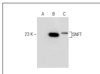
SNFT (M-13): sc-162246. Western blot analysis of SNFT expression in non-transfected 293T: sc-117752 (A), human SNFT transfected 293T: sc-373308 (B) and TK-1 (C) whole cell lysates.
