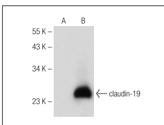
claudin-19 (C-12): sc-162687. Western blot analysis of claudin-19 expression in non-transfected: sc-117752 (A) and human claudin-19 transfected: sc-114824 (B) 293T whole cell lysates.
