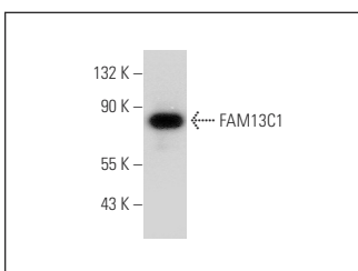
FAM13C1 (S-15): sc-162793. Western blot analysis of FAM13C1 expression in rat brain tissue extract.
