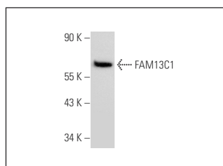
FAM13C1 (T-13): sc-162794. Western blot analysis of FAM13C1 expression in LADMAC whole cell lysate.
