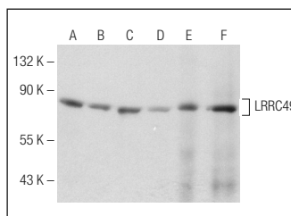
LRRC49 (G-15): sc-163039. Western blot analysis of LRRC49 expression in HeLa (A), U-87 MG (B), Hep G2 (C) and DU 145 (D) whole cell lysates and rat brain (E) and mouse brain (F) tissue extracts.
