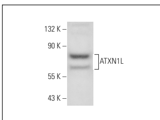
ATXN1L (N-12): sc-163714. Western blot analysis of ATXN1L expression in U-251-MG whole cell lysate.
