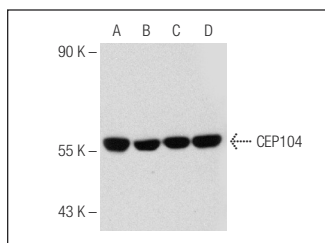
CEP104 (N-14): sc-164761. Western blot analysis of CEP104 expression in HeLa (A), MOLT-4 (B), SK-BR-3 (C) and Hep G2 (D) whole cell lysates.
