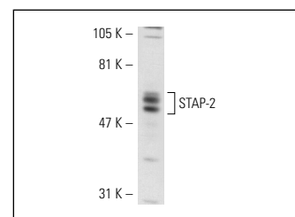
STAP-2 (C-20): sc-16521. Western blot analysis of STAP-2 expression in T-47D whole cell lysate.
