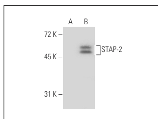
STAP-2 (C-20): sc-16521. Western blot analysis of STAP-2 expression in non-transfected: sc-110760 (A) and human STAP-2 transfected: sc-110839 (B) 293 whole cell lysates.
