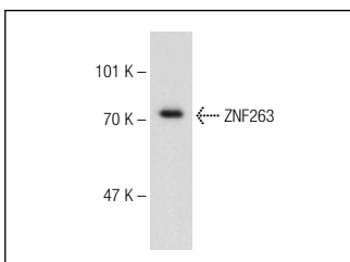
ZNF263 (T-14): sc-165960. Western blot analysis of ZNF263 expression in HeLa nuclear extract.
