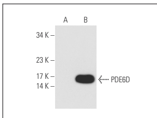
PDE6D (C-8): sc-166855. Western blot analysis of PDE6D expression in non-transfected: sc-117752 (A) and mouse PDE6D transfected: sc-122458 (B) 293T whole cell lysates.
