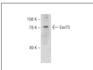
Exo70 (D-16): sc-167766. Western blot analysis of Exo70 expression in Jurkat whole cell lysate.
